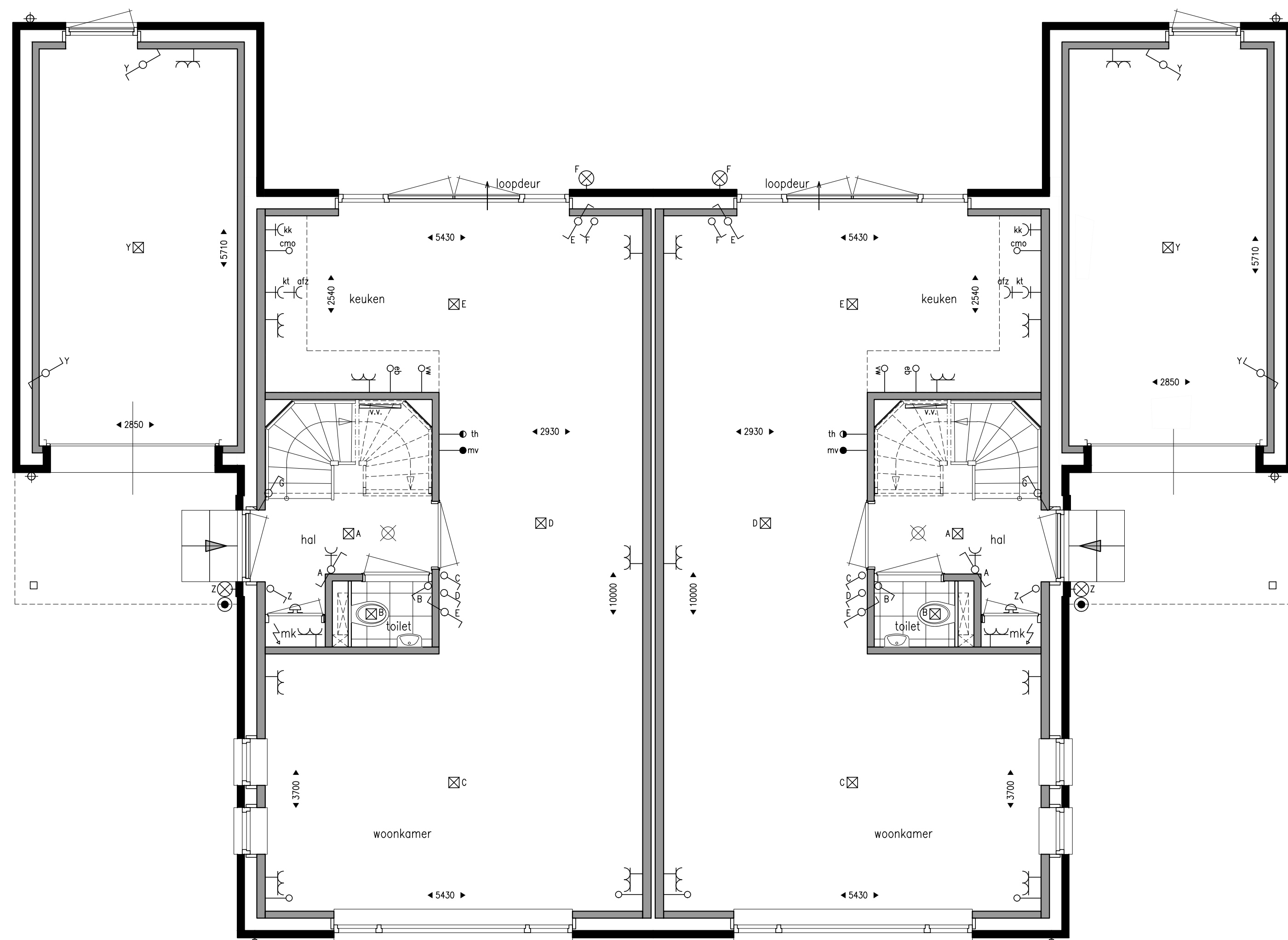
Type E Type E BEGANE GROND 1:50
